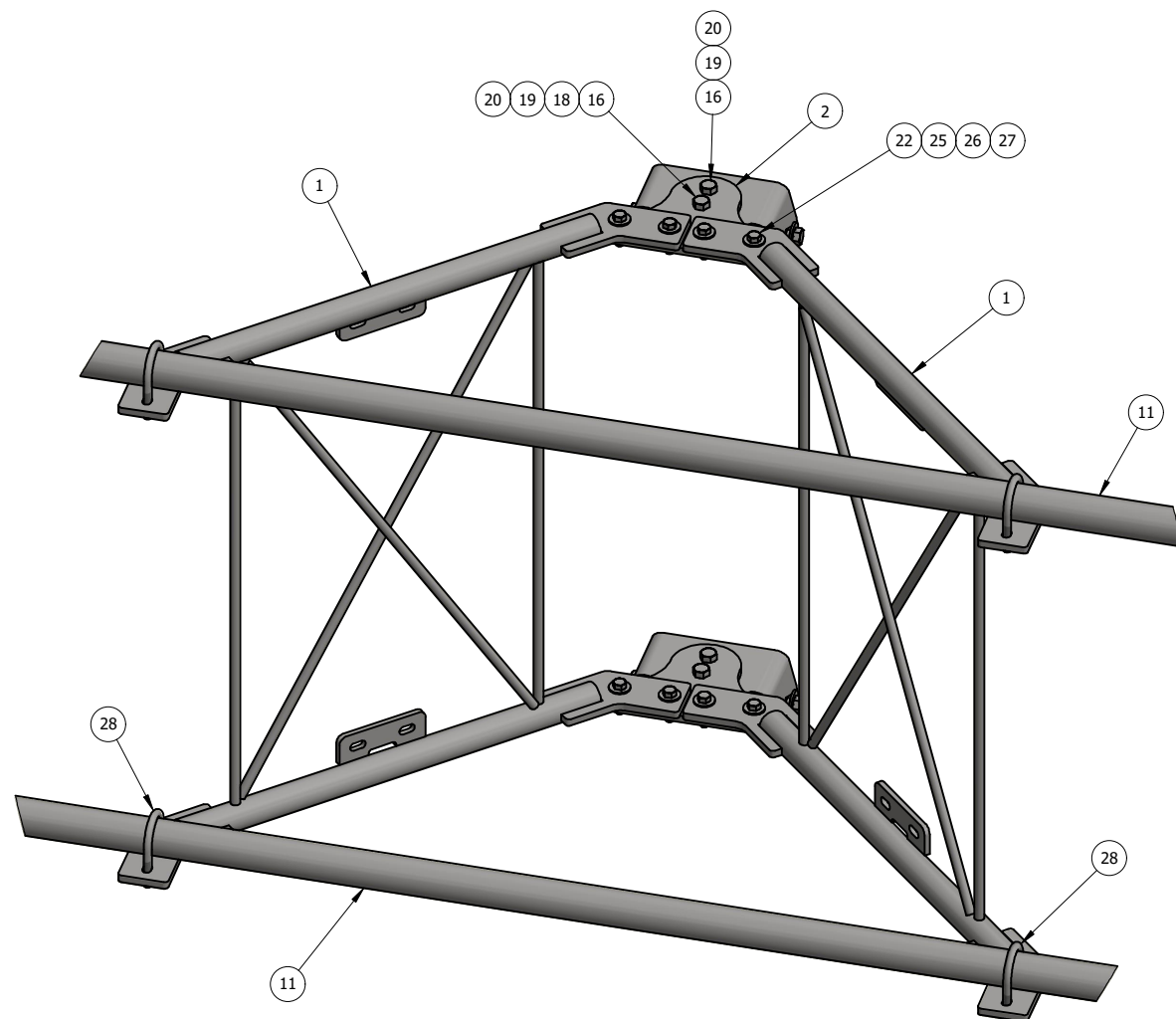
V-FRAME - DETAIL
