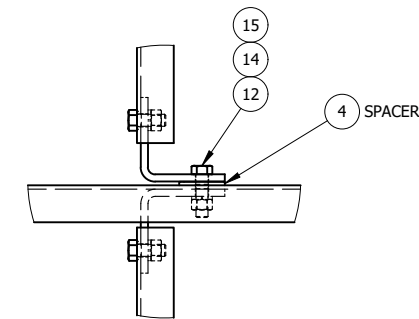
DETAIL - D
