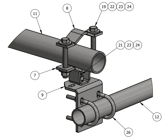
DETAIL - C STIFF ARM PIPE FACE CONNECTION
