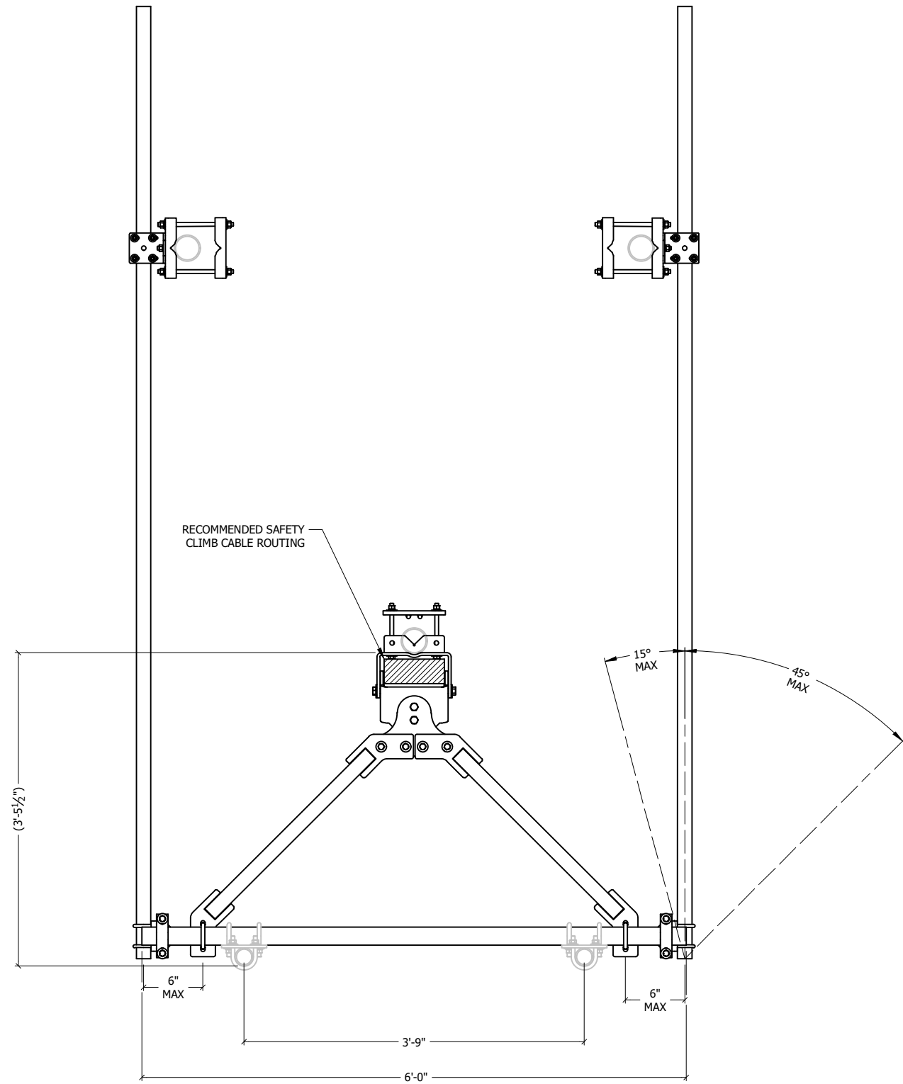
TOP VIEW
