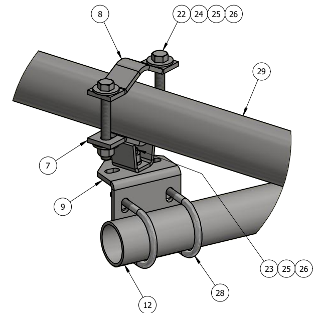
DETAIL - C STIFF ARM PIPE FACE CONNECTION
