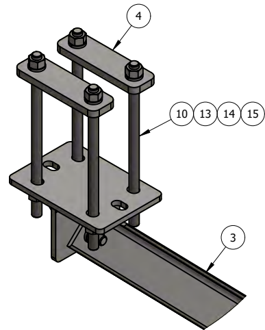
DETAIL - B
