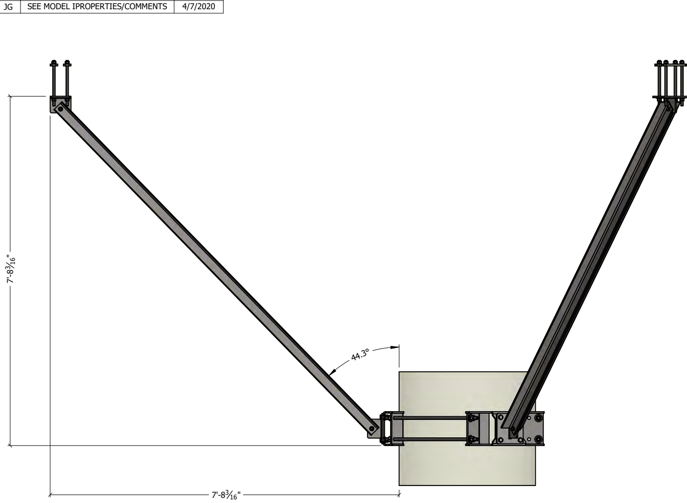
SIDE VIEW
