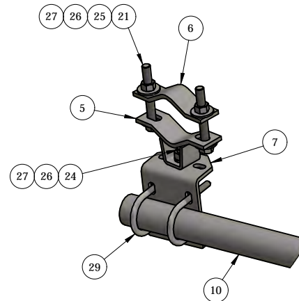
DETAIL - C STIFF ARM PIPE FACE CONNECTION
