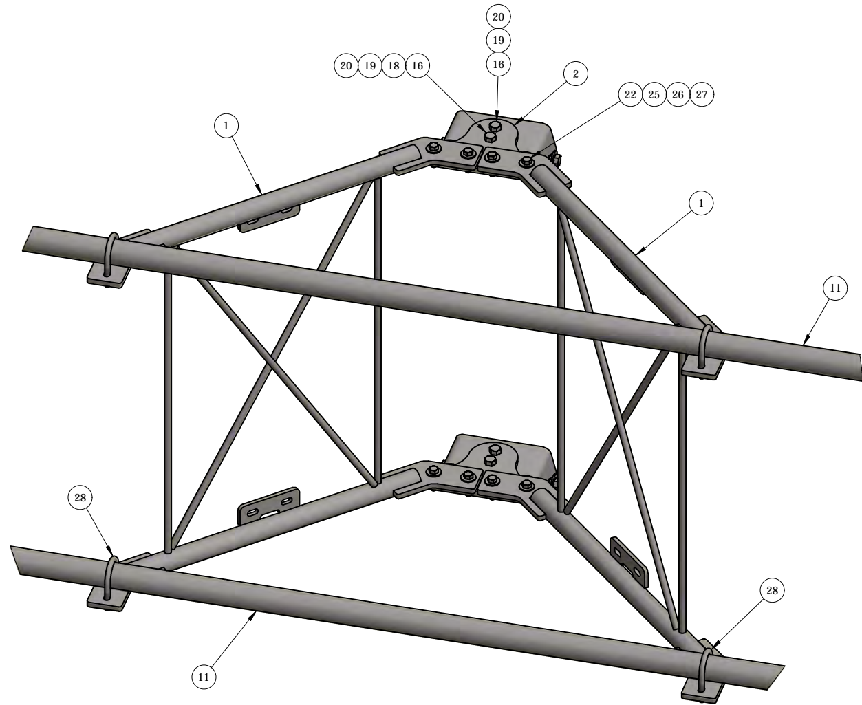
V-FRAME - DETAIL
