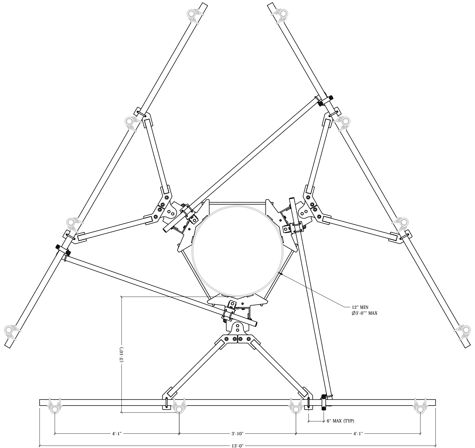
TOP VIEW
