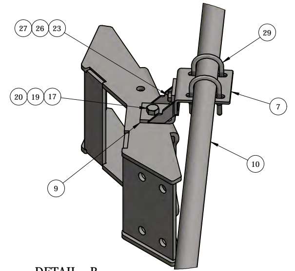
DETAIL - B STIFF ARM RING MOUNT CONNECTION
