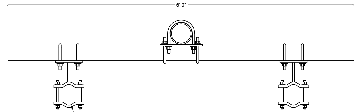
TOP VIEW
