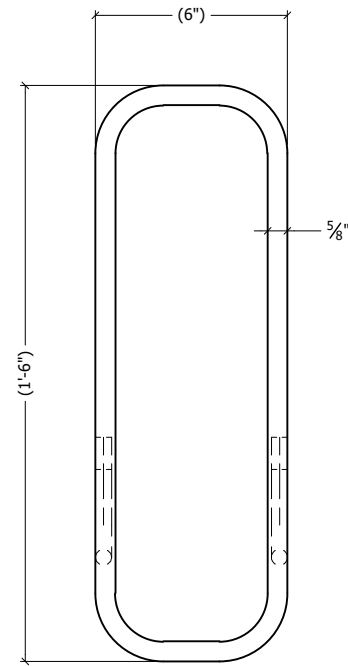
FRONT VIEW
