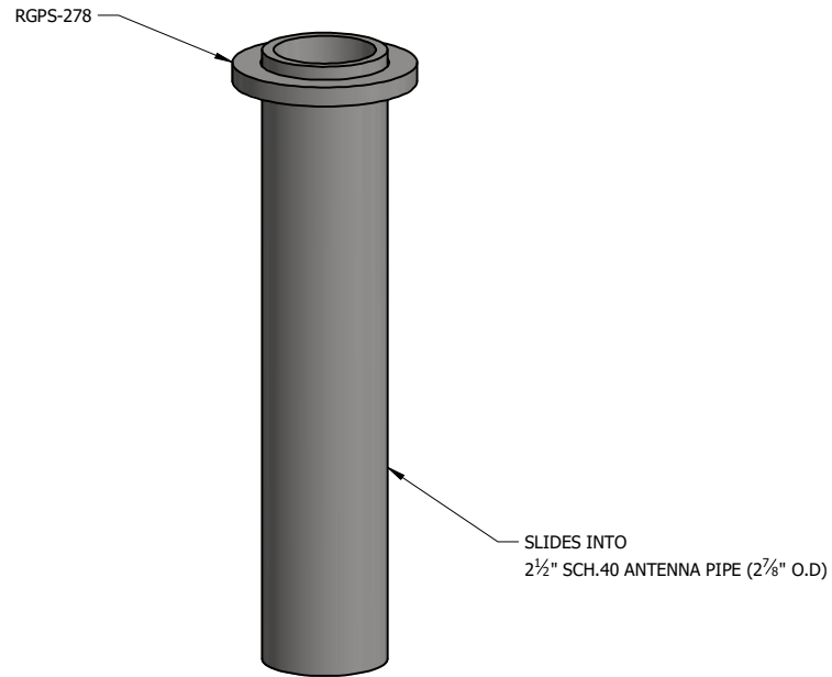
DETAIL - A
