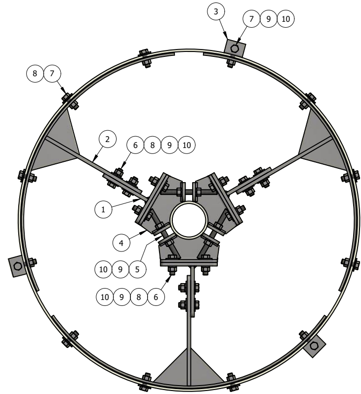
TOP VIEW CAP PL NOT SHOWN FOR CLARITY
