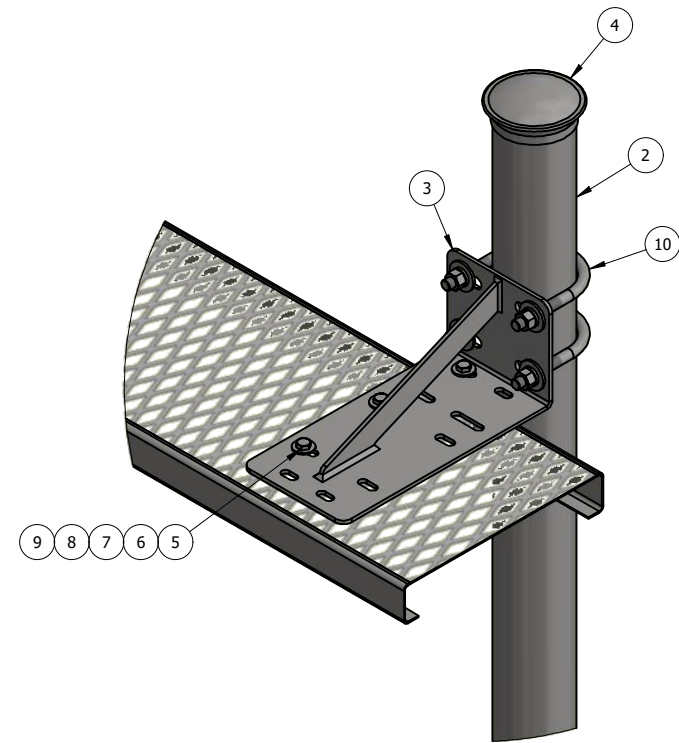
DETAIL - A
