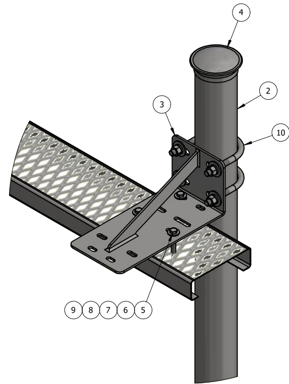
DETAIL - A
