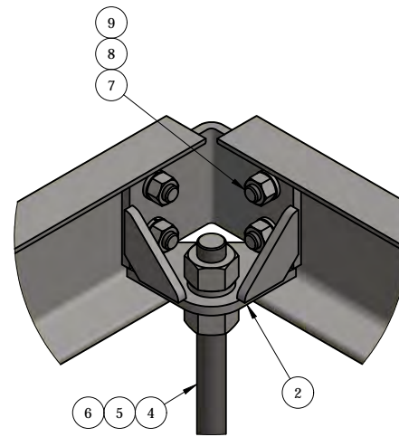
DETAIL - A
