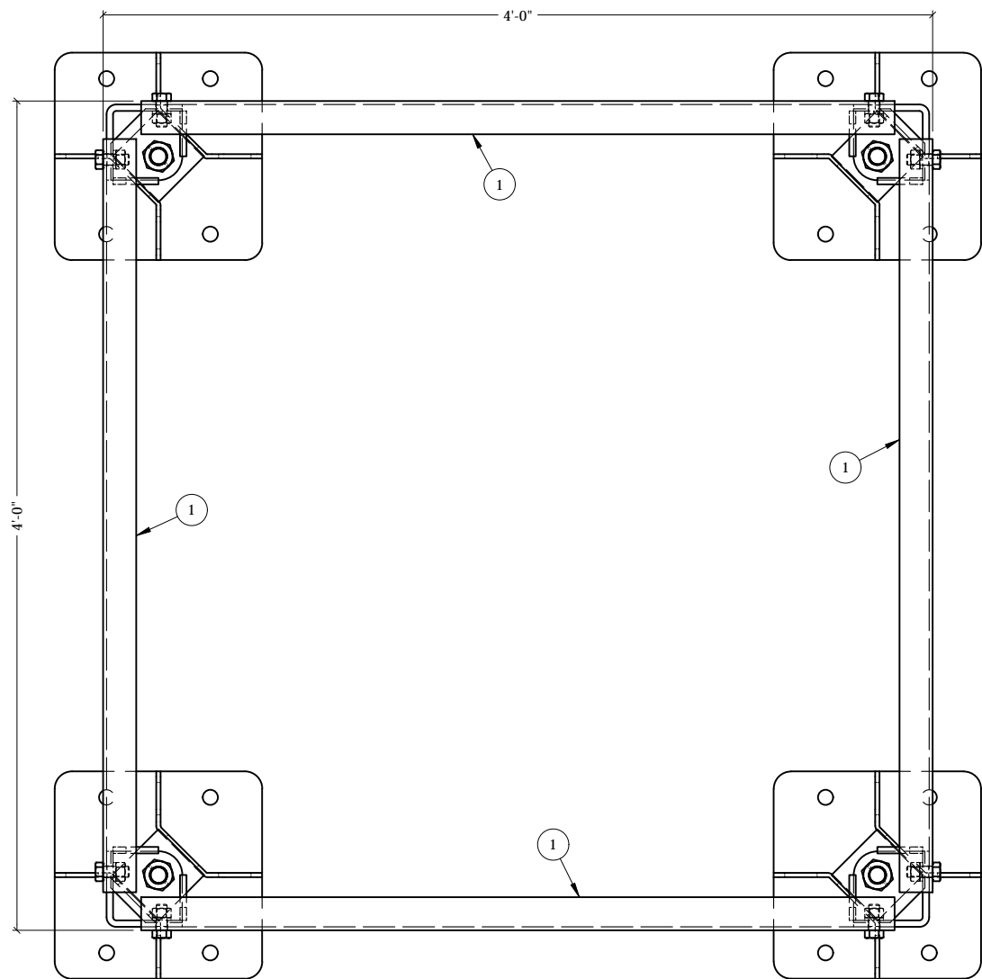
PLAN VIEW
