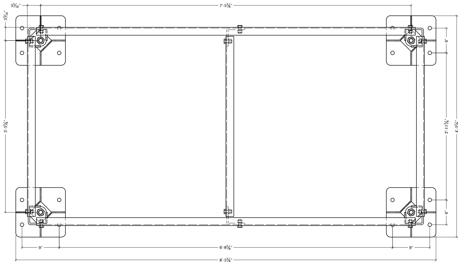
FOOT PAD LAYOUT
