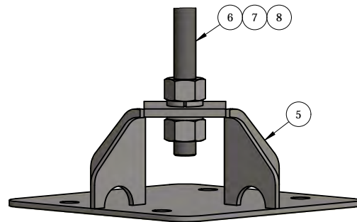
DETAIL - C
