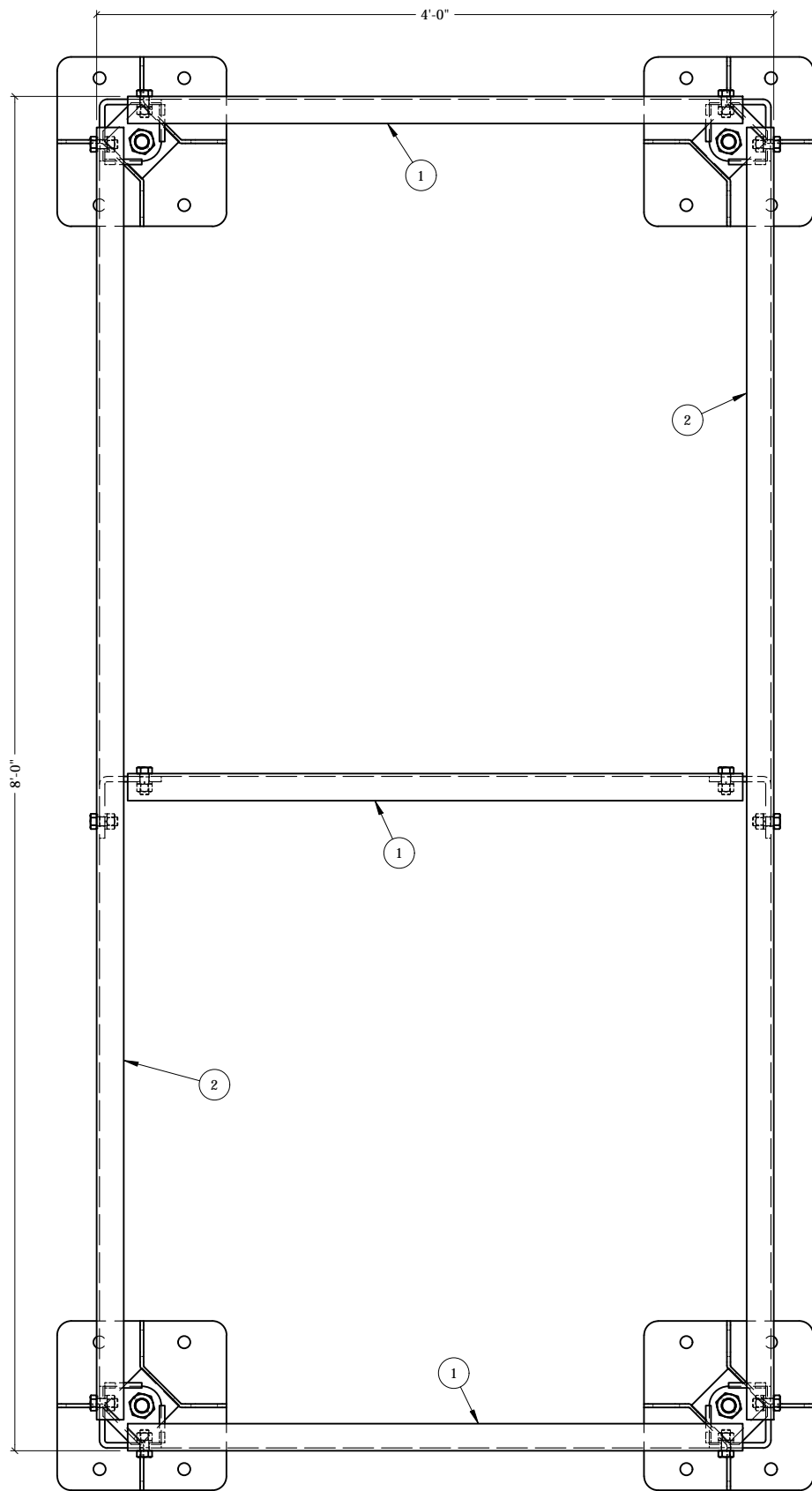
PLAN VIEW
