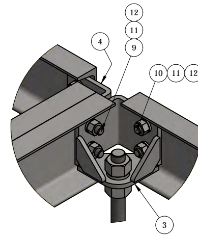
DETAIL - B
