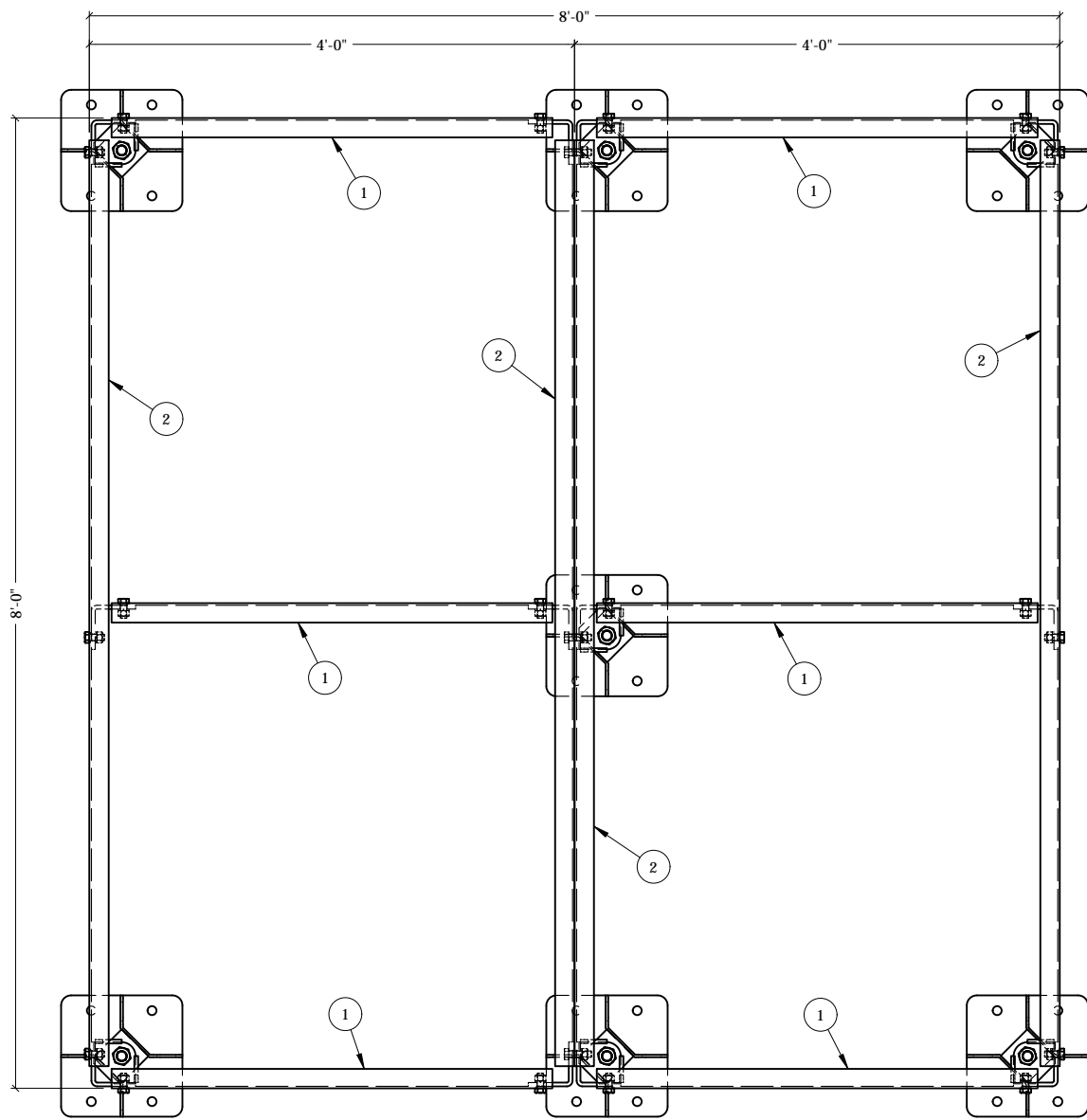
PLAN VIEW
