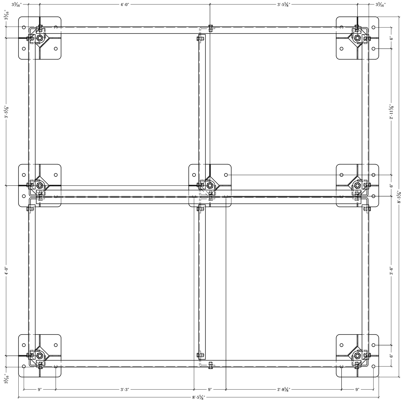
FOOT PAD LAYOUT
