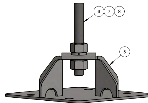
DETAIL - C
