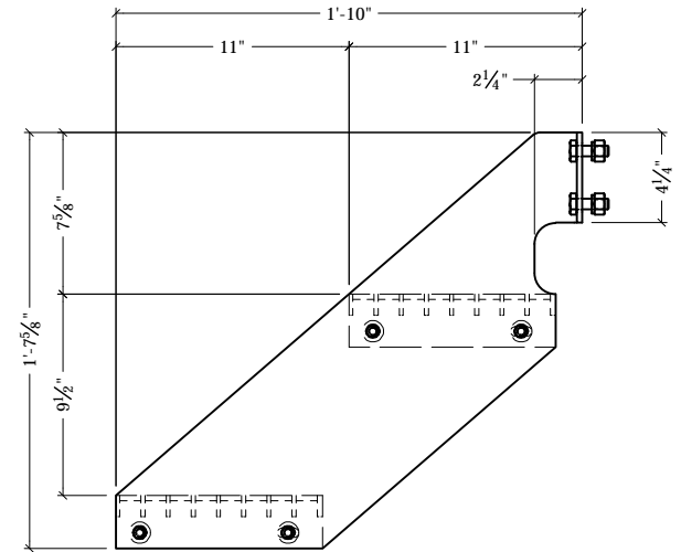
SIDE VIEW MAX RISE NOT TO EXCEED 9 1/2" WHEN MOUNTED
