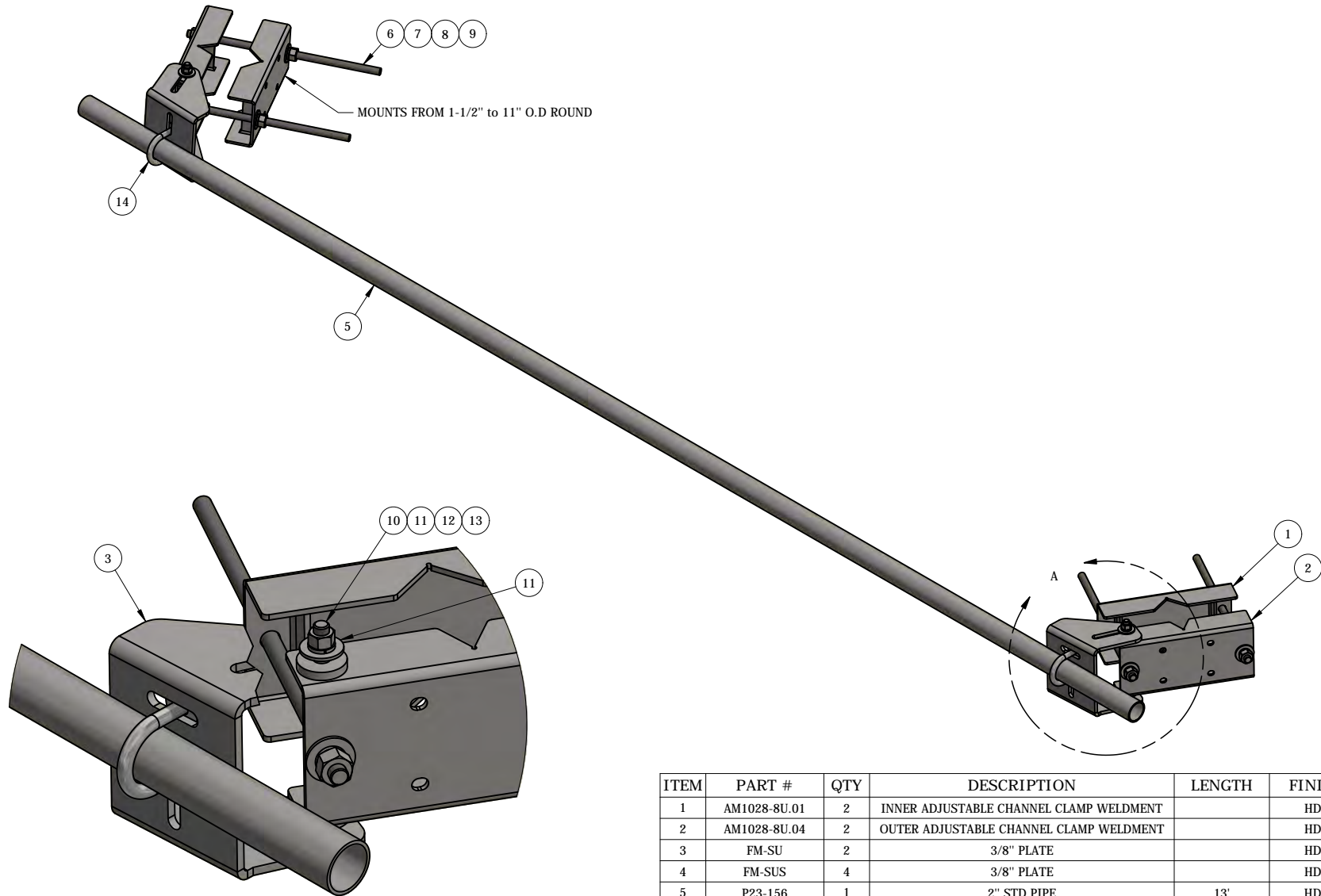
DETAIL - A
