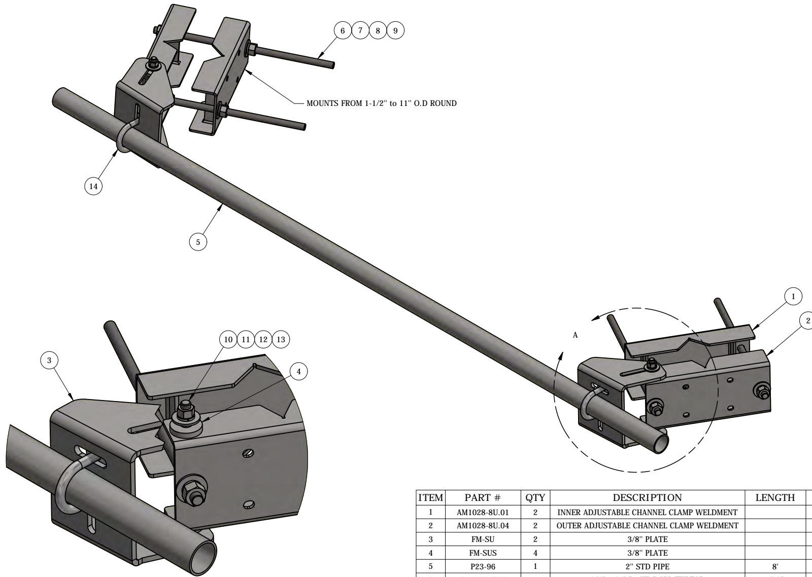
DETAIL - A
