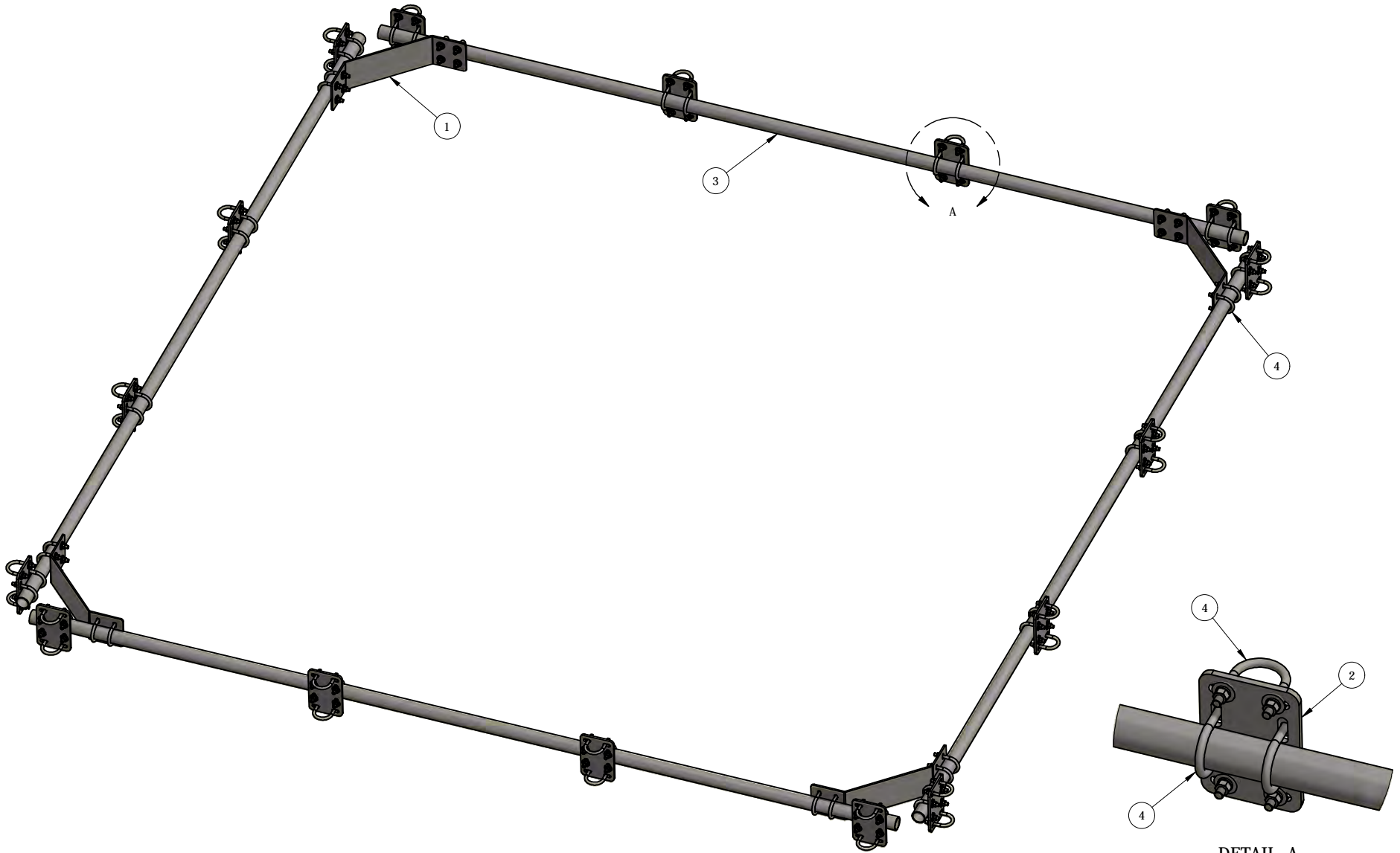
DETAIL A
