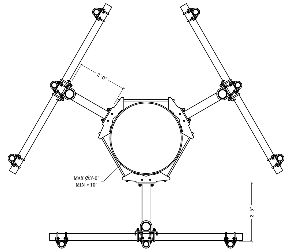
TOP VIEW
