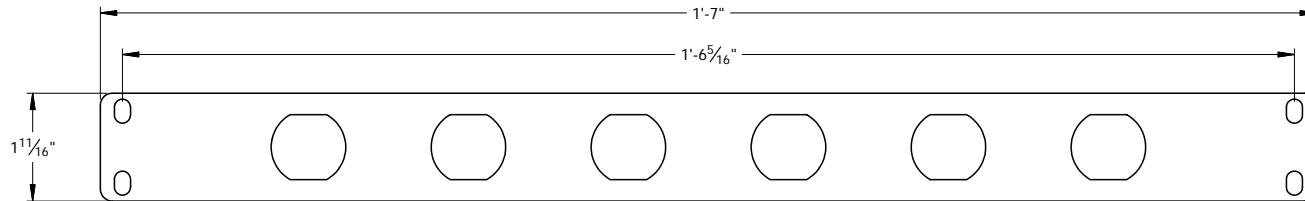
FRONT VIEW
