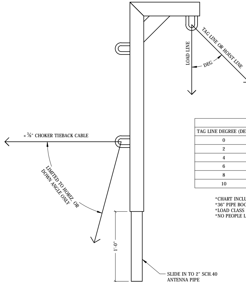
SIDE VIEW
