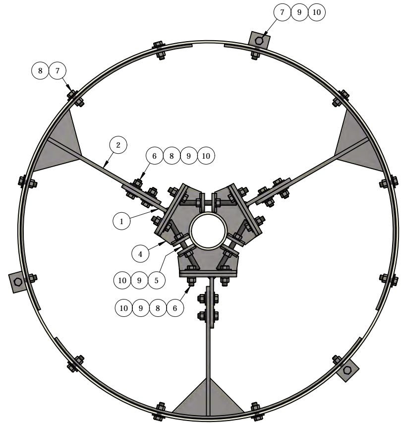
TOP VIEW CAP PL NOT SHOWN FOR CLARITY
