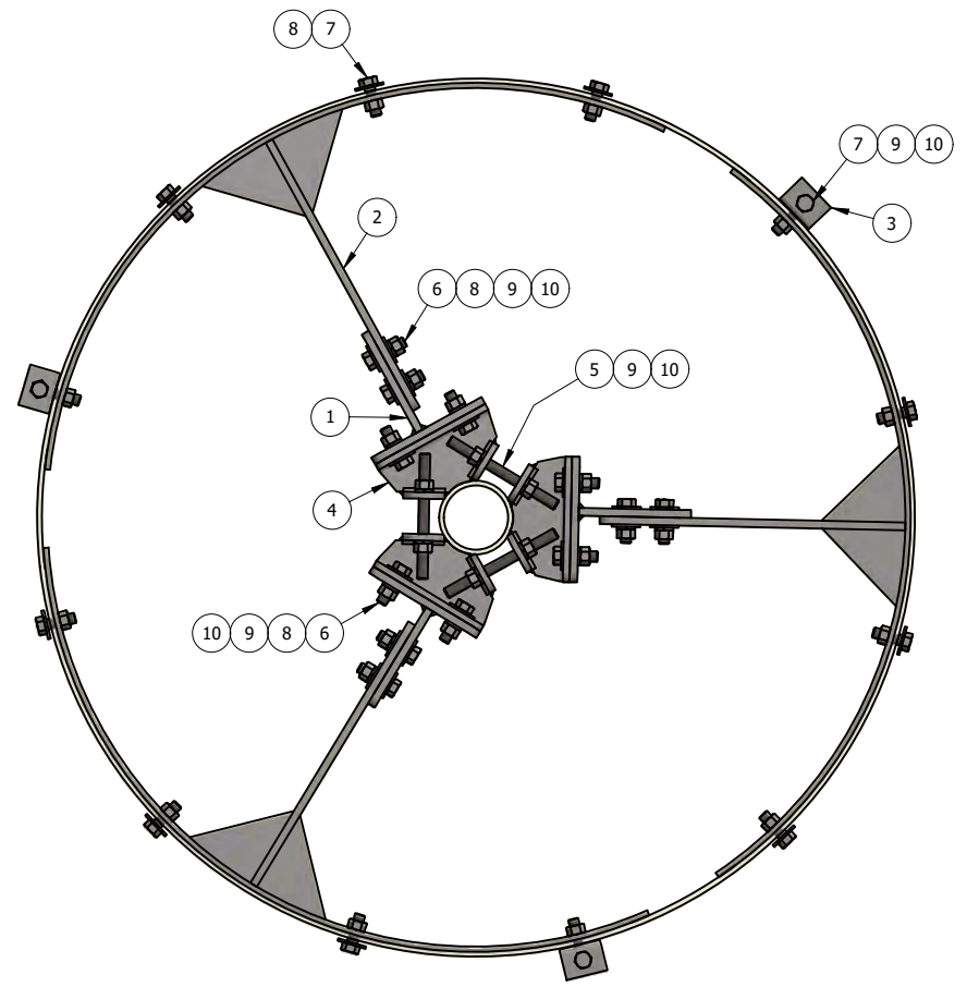
TOP VIEW CAP PL NOT SHOWN FOR CLARITY
