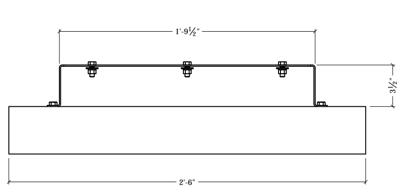
END VIEW
