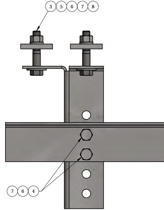
DETAIL-A
