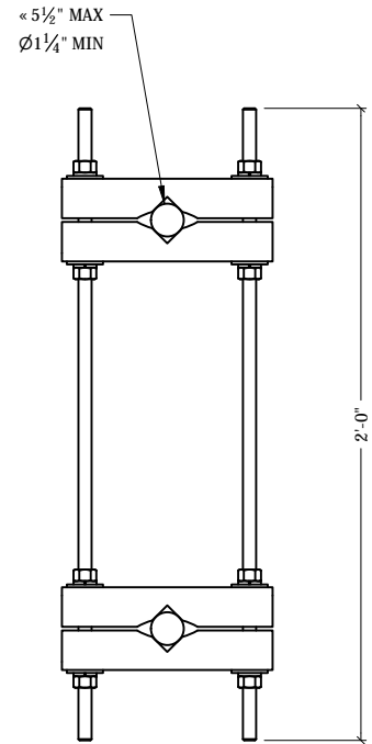
TOP VIEW
