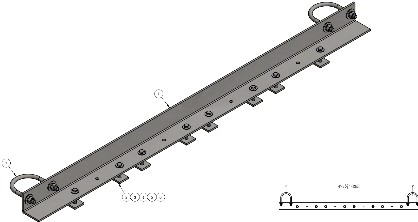
TOP VIEW
